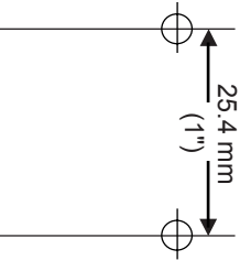
Wall mount template for the charger
